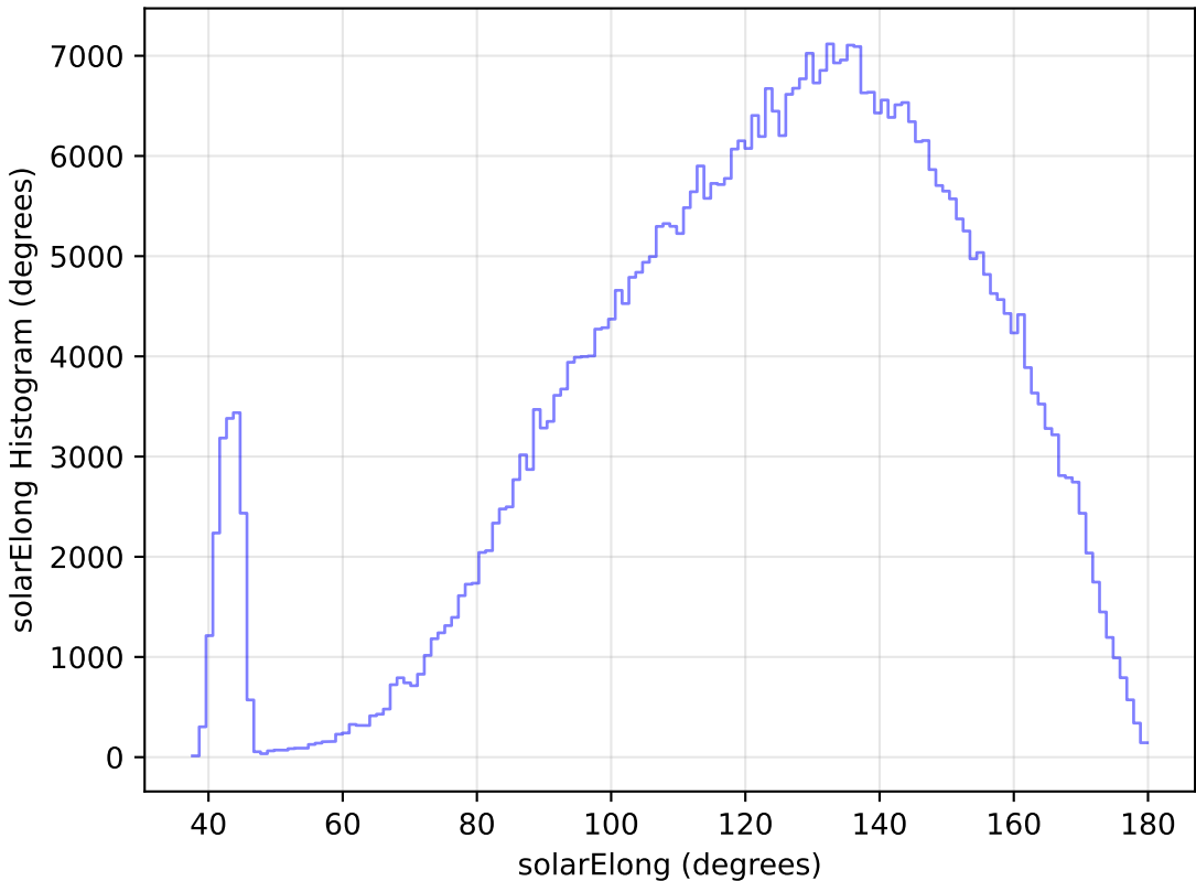
too_elab_r16_d2_giz_v3.4_10yrs WFD r band: solarElong Histogram
