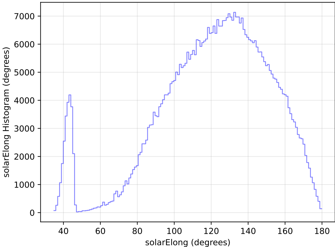
too_elab_r16_d2_giz_v3.4_10yrs WFD i band: solarElong Histogram
