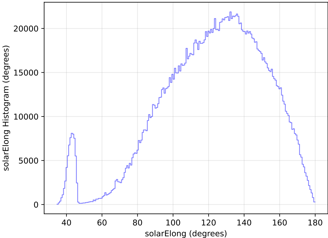
too_elab_r16_d2_giz_v3.4_10yrs WFD all bands: solarElong Histogram
