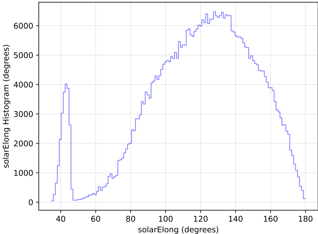
too_elab_r16_d2_giz_v3.4_10yrs All sky z band: solarElong Histogram
