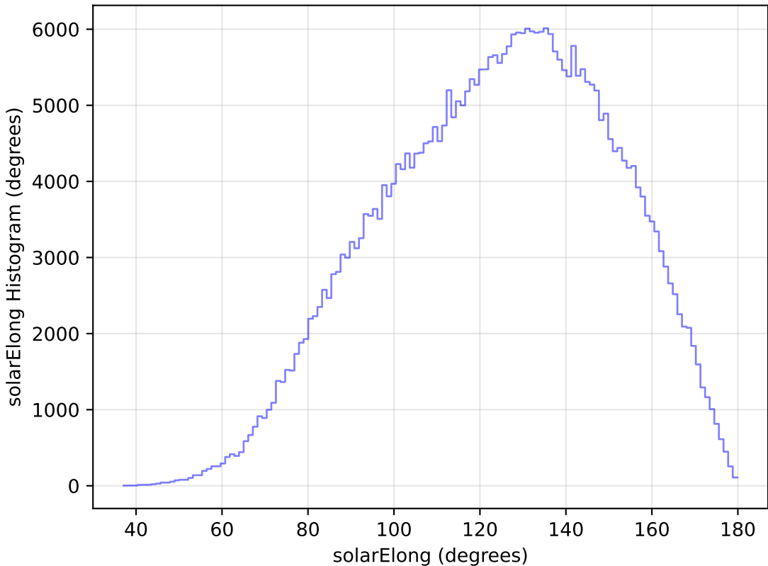
too_elab_r16_d2_giz_v3.4_10yrs All sky y band: solarElong Histogram
