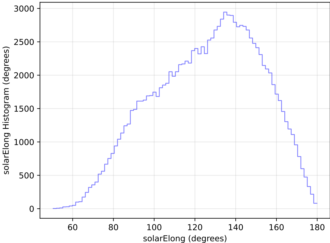
too_elab_r16_d2_giz_v3.4_10yrs All sky u band: solarElong Histogram
