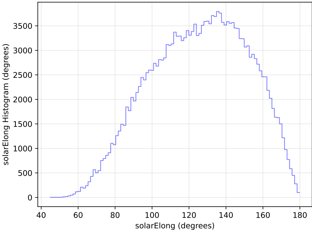
too_elab_r16_d2_giz_v3.4_10yrs All sky g band: solarElong Histogram
