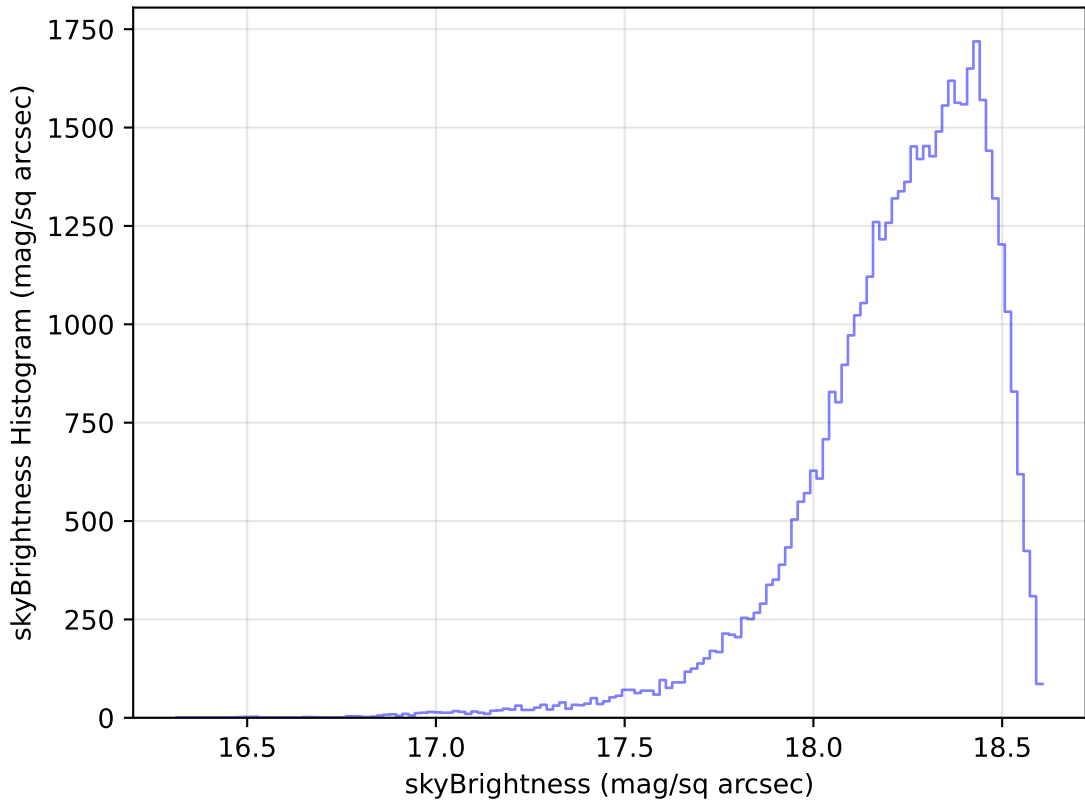
too_elab_r16_d2_giz_v3.4_10yrs Yr 1 y band: skyBrightness Histogram
