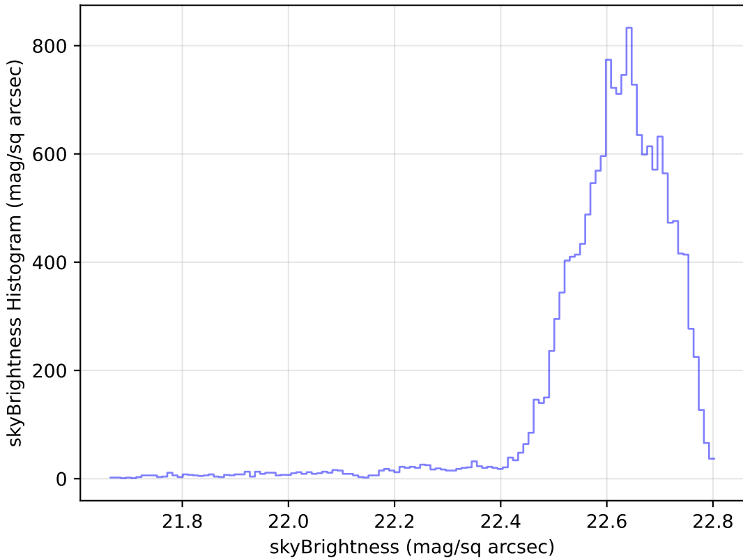
too_elab_r16_d2_giz_v3.4_10yrs Yr 1 u band: skyBrightness Histogram
