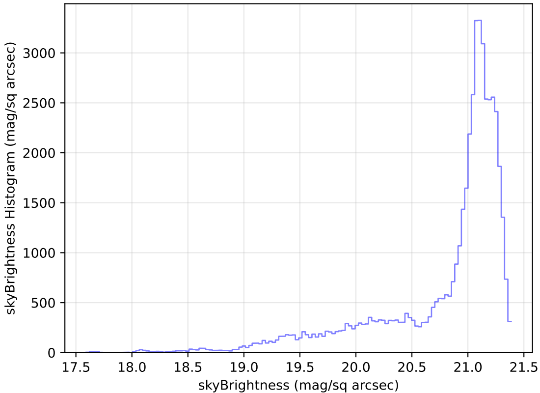
too_elab_r16_d2_giz_v3.4_10yrs Yr 1 r band: skyBrightness Histogram
