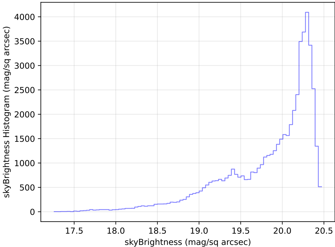
too_elab_r16_d2_giz_v3.4_10yrs Yr 1 i band: skyBrightness Histogram
