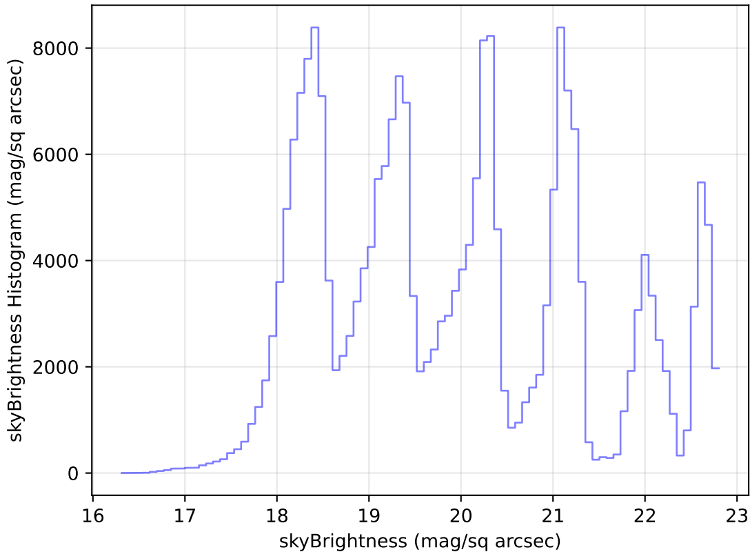
too_elab_r16_d2_giz_v3.4_10yrs Yr 1 all bands: skyBrightness Histogram
