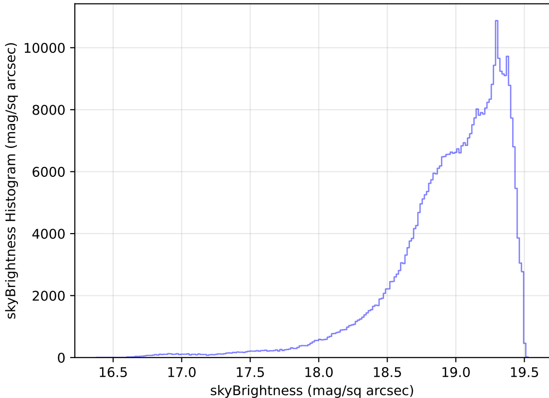
too_elab_r16_d2_giz_v3.4_10yrs WFD z band: skyBrightness Histogram
