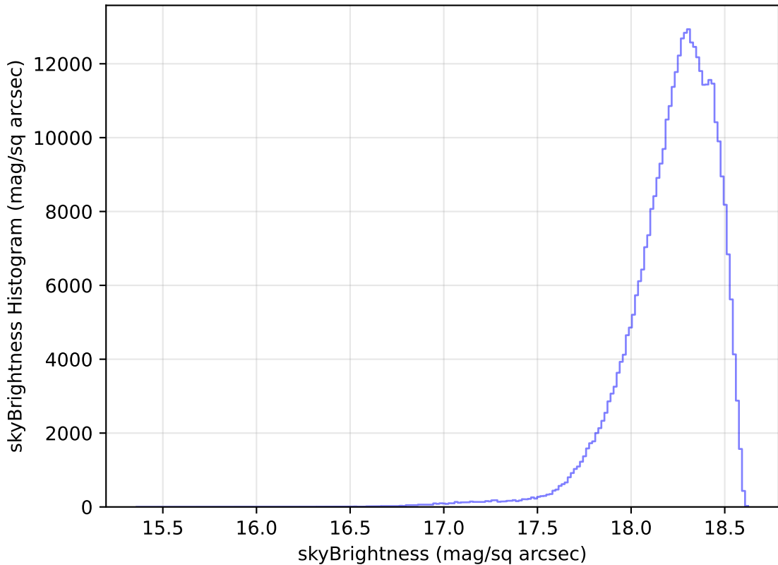
too_elab_r16_d2_giz_v3.4_10yrs WFD y band: skyBrightness Histogram
