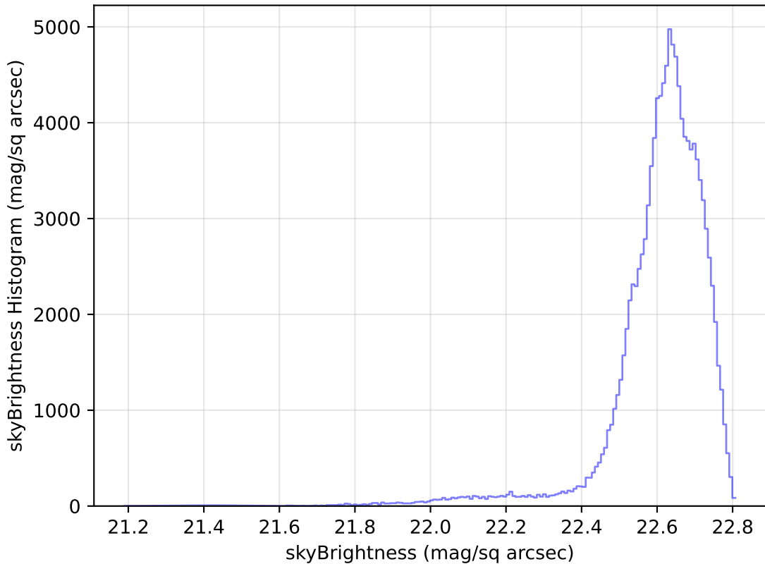
too_elab_r16_d2_giz_v3.4_10yrs WFD u band: skyBrightness Histogram
