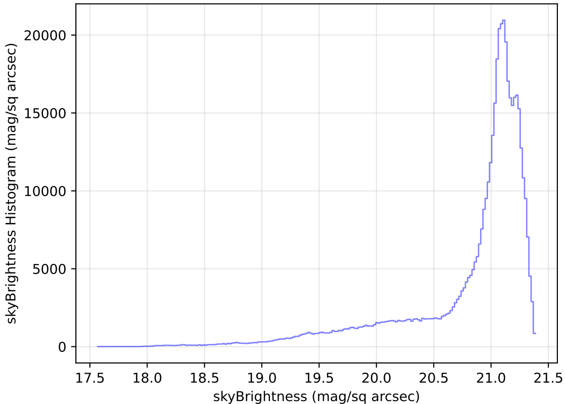
too_elab_r16_d2_giz_v3.4_10yrs WFD r band: skyBrightness Histogram
