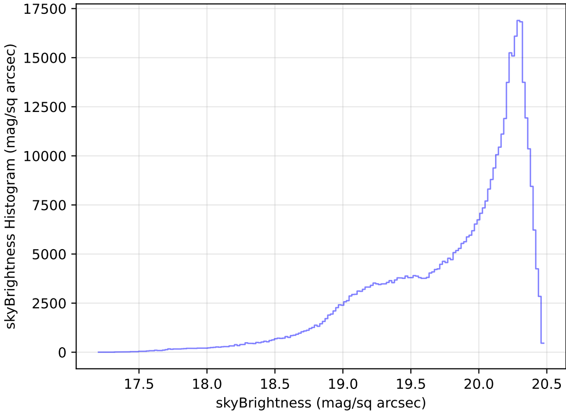
too_elab_r16_d2_giz_v3.4_10yrs WFD i band: skyBrightness Histogram
