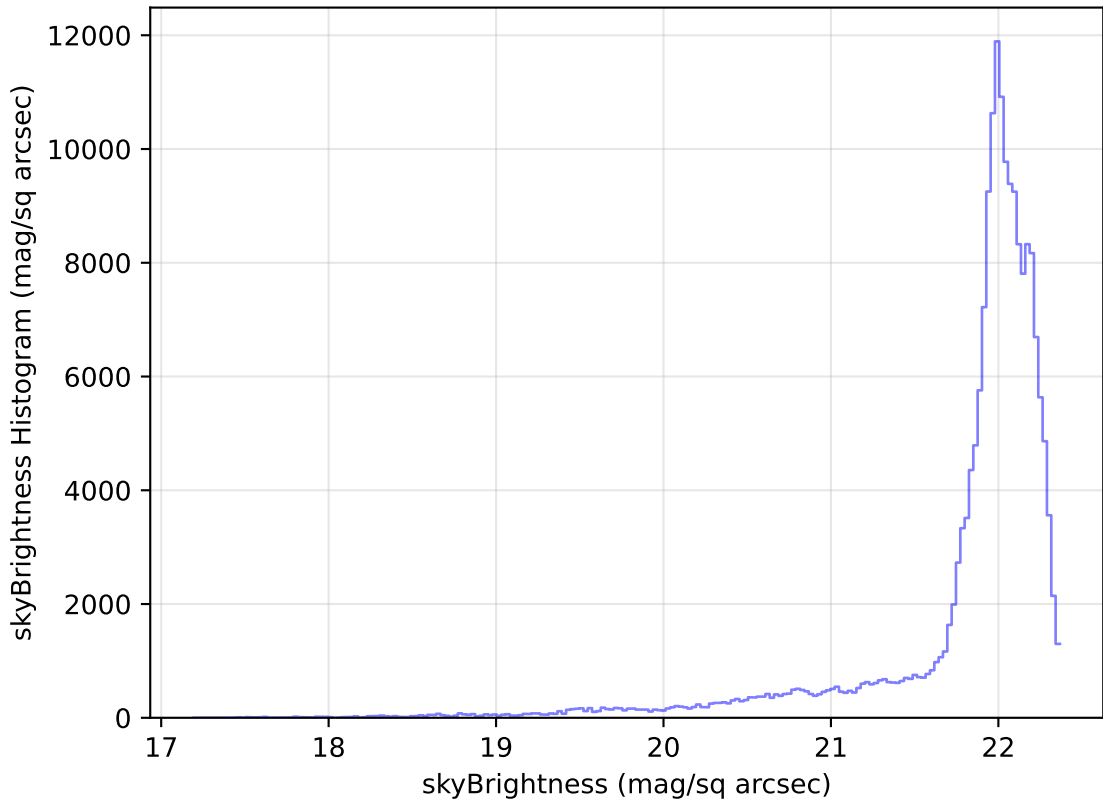
too_elab_r16_d2_giz_v3.4_10yrs WFD g band: skyBrightness Histogram
