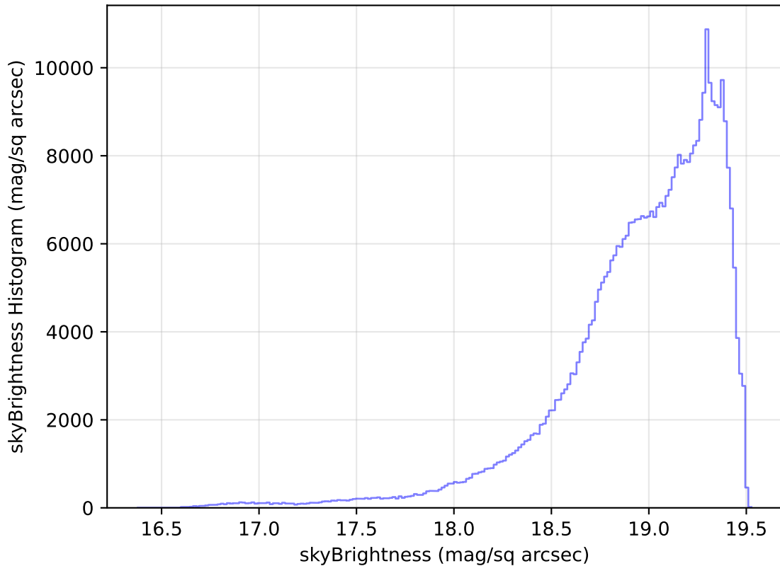
too_elab_r16_d2_giz_v3.4_10yrs All sky z band: skyBrightness Histogram
