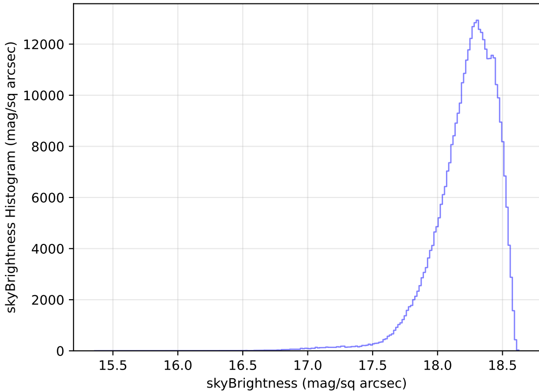
too_elab_r16_d2_giz_v3.4_10yrs All sky y band: skyBrightness Histogram
