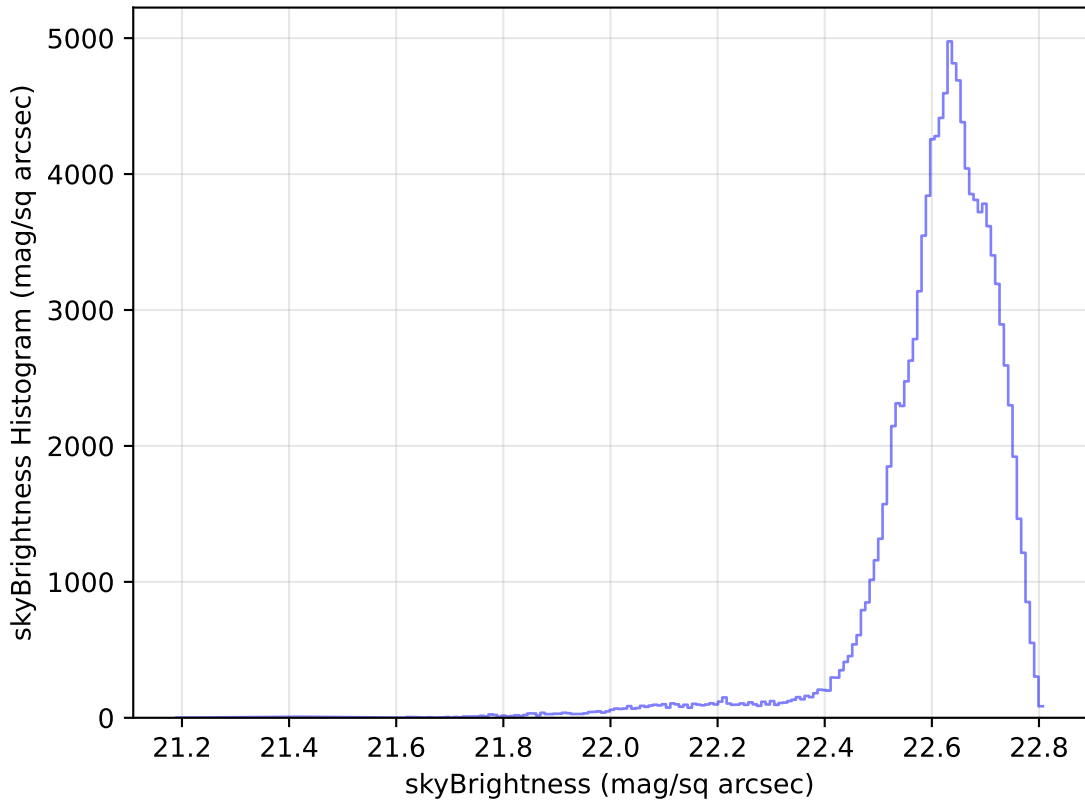
too_elab_r16_d2_giz_v3.4_10yrs All sky u band: skyBrightness Histogram
