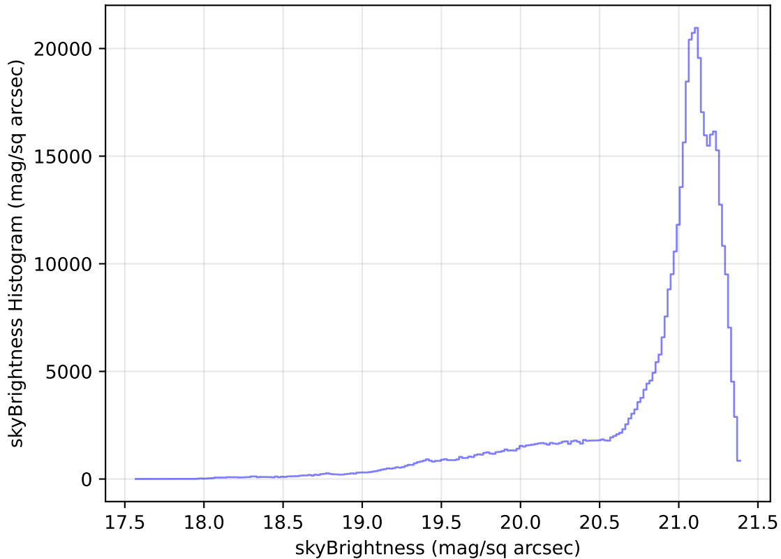
too_elab_r16_d2_giz_v3.4_10yrs All sky r band: skyBrightness Histogram
