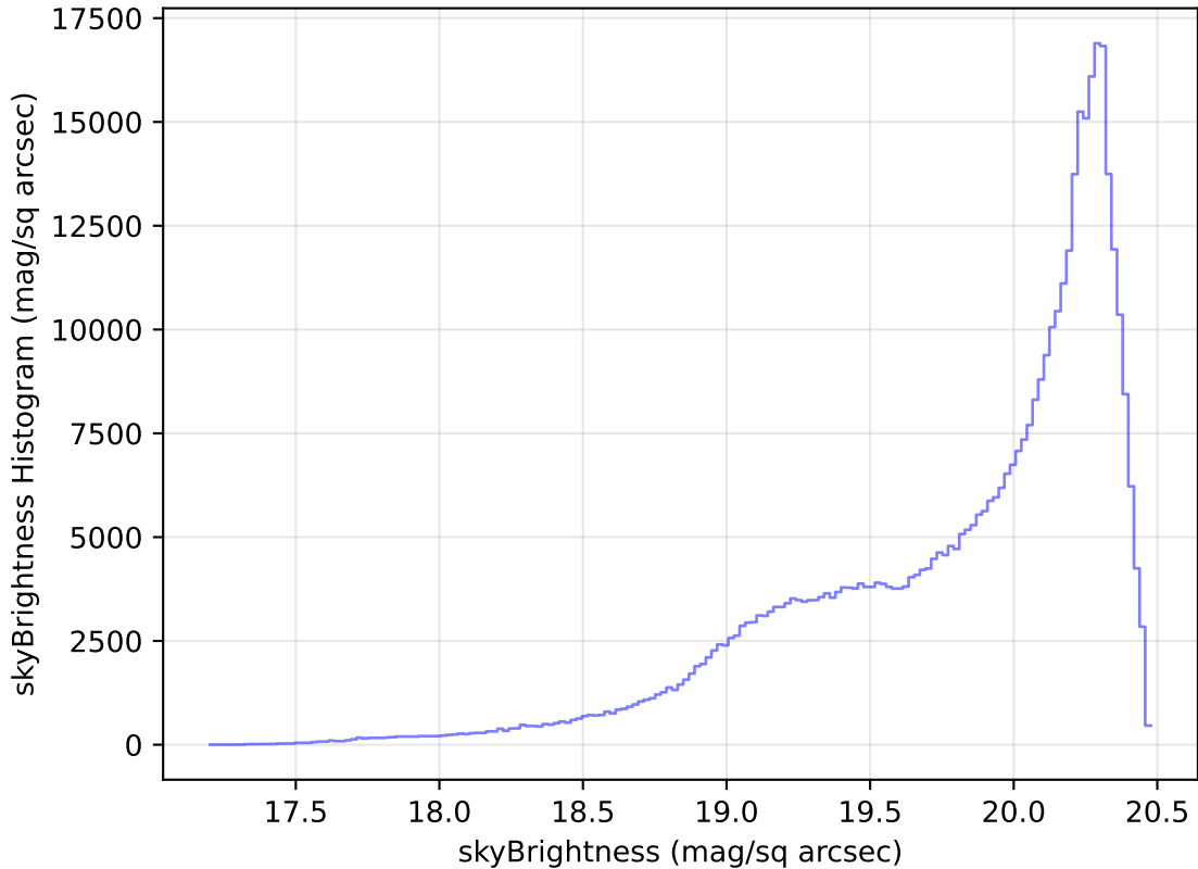
too_elab_r16_d2_giz_v3.4_10yrs All sky i band: skyBrightness Histogram
