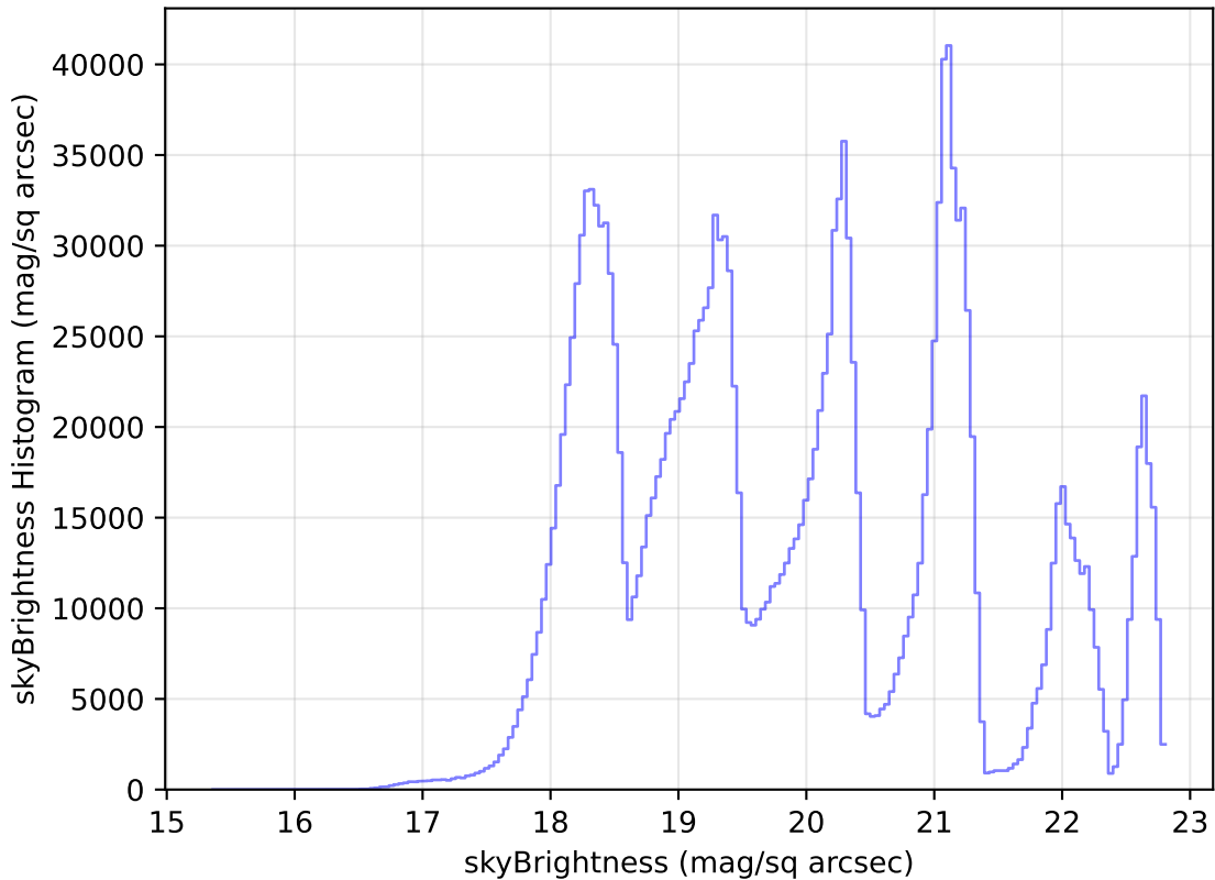
too_elab_r16_d2_giz_v3.4_10yrs All sky all bands: skyBrightness Histogram
