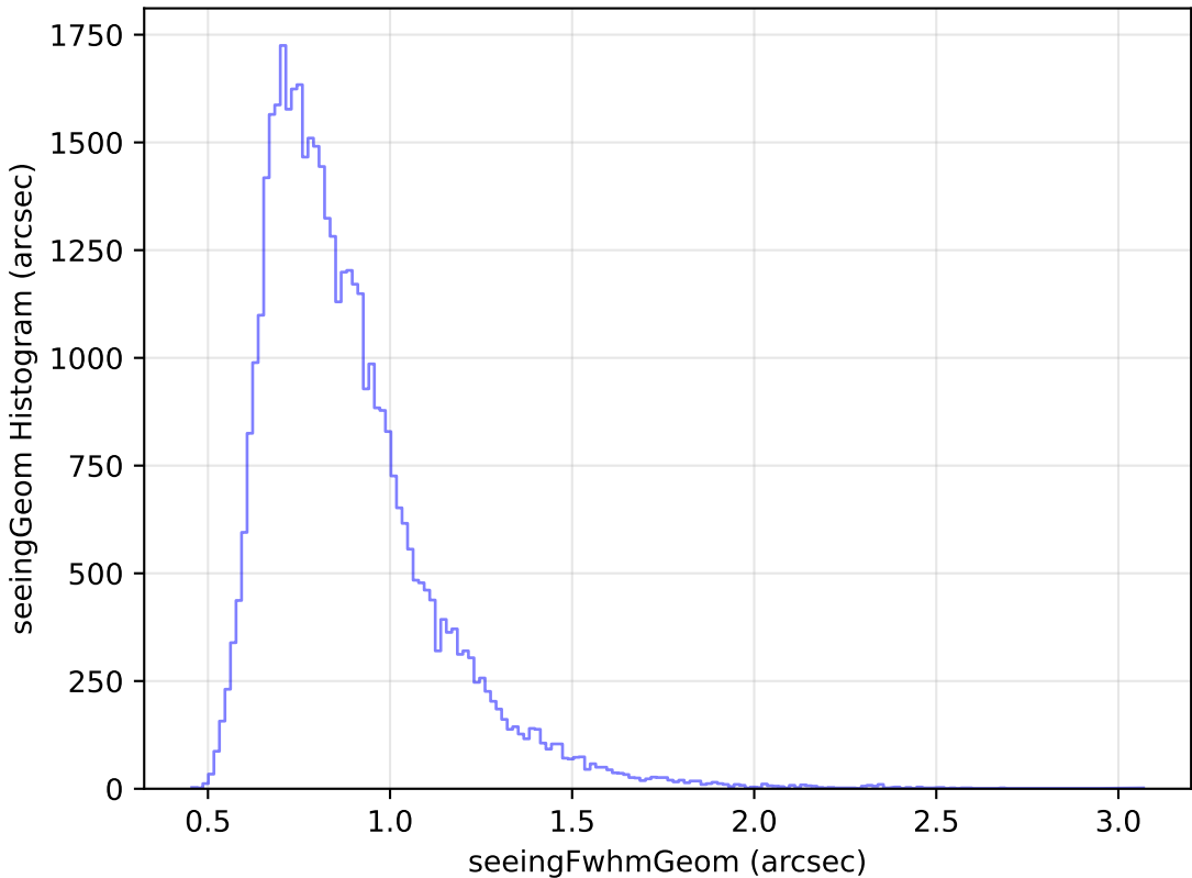
too_elab_r16_d2_giz_v3.4_10yrs Yr 1 z band: seeingGeom Histogram
