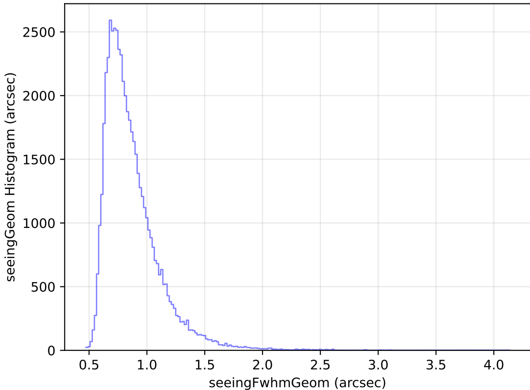
too_elab_r16_d2_giz_v3.4_10yrs Yr 1 i band: seeingGeom Histogram
