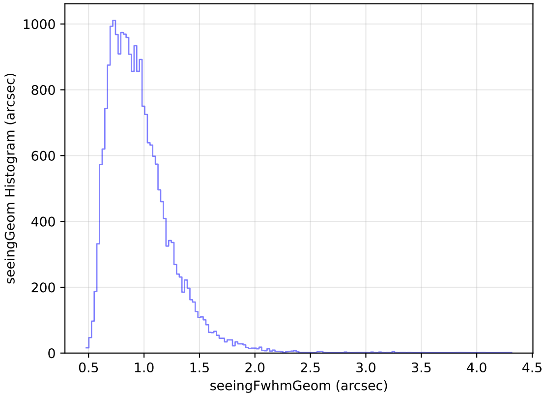
too_elab_r16_d2_giz_v3.4_10yrs Yr 1 g band: seeingGeom Histogram
