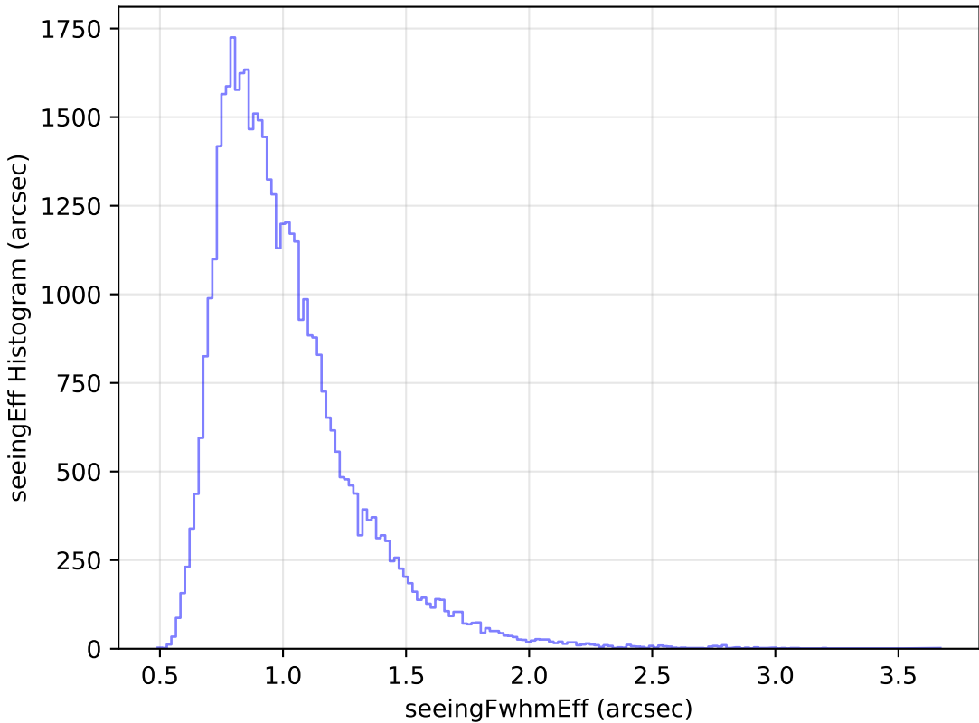
too_elab_r16_d2_giz_v3.4_10yrs Yr 1 z band: seeingEff Histogram
