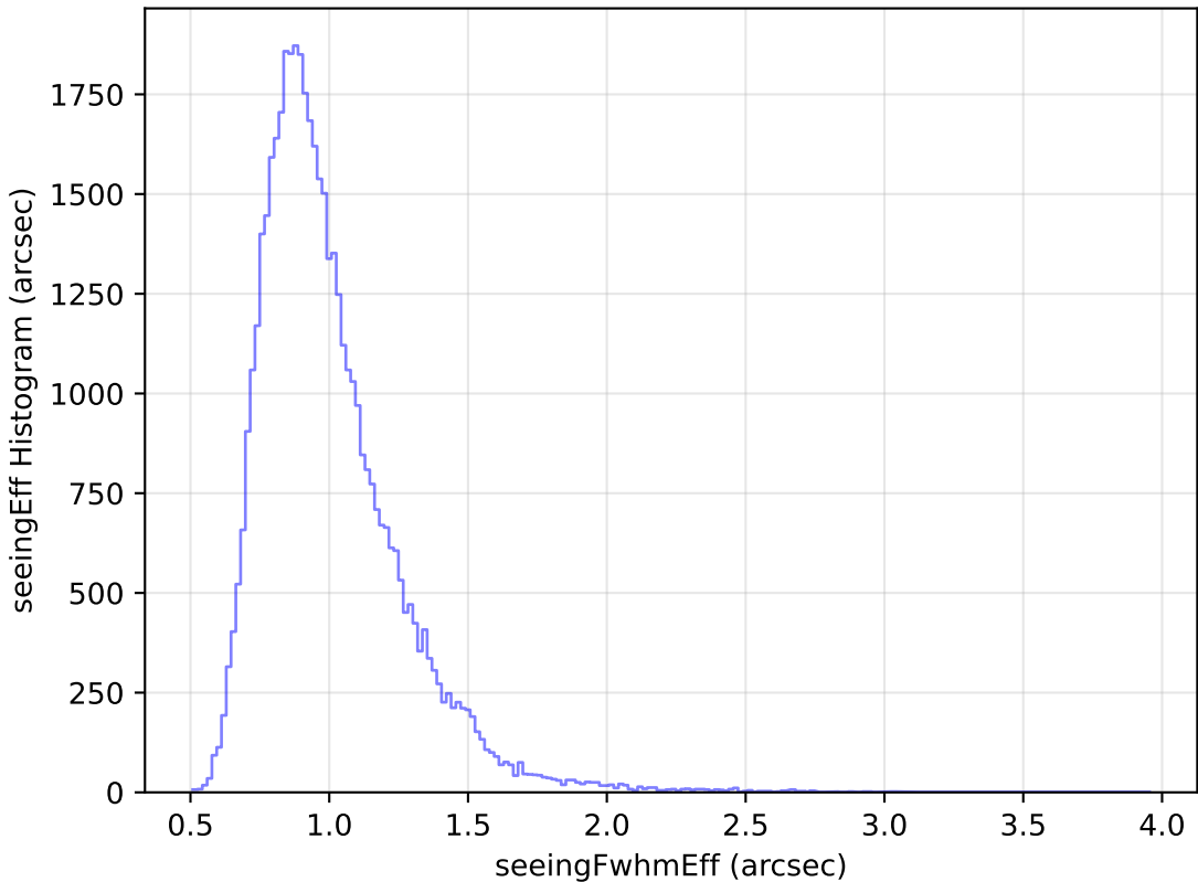
too_elab_r16_d2_giz_v3.4_10yrs Yr 1 y band: seeingEff Histogram
