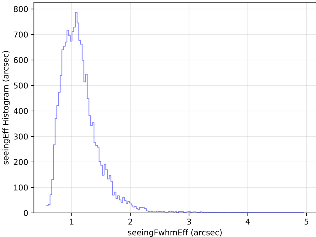
too_elab_r16_d2_giz_v3.4_10yrs Yr 1 u band: seeingEff Histogram
