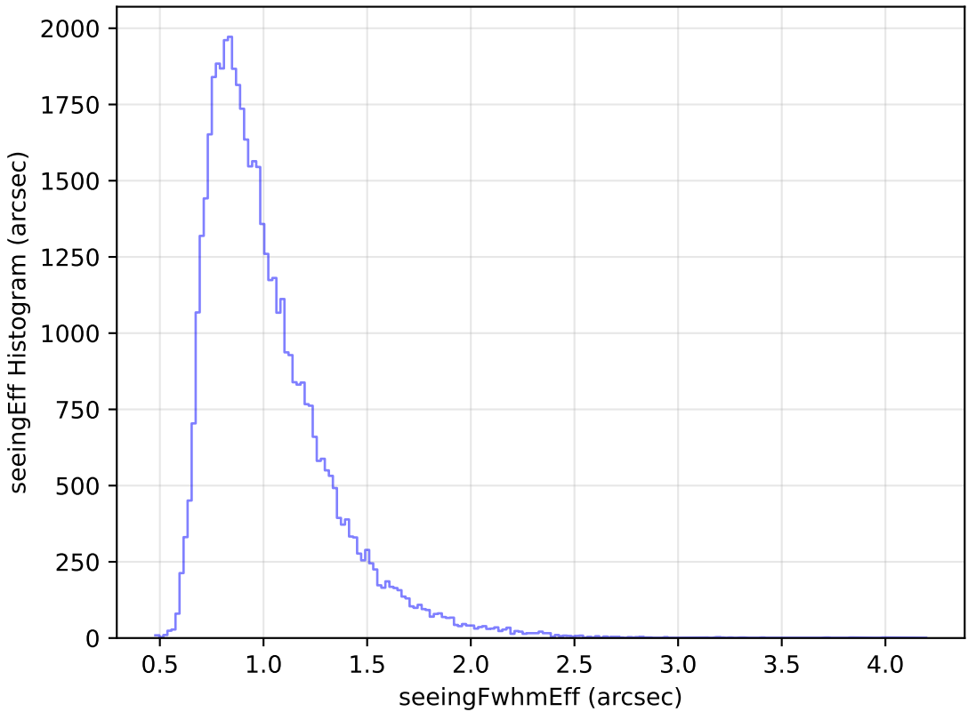
too_elab_r16_d2_giz_v3.4_10yrs Yr 1 r band: seeingEff Histogram
