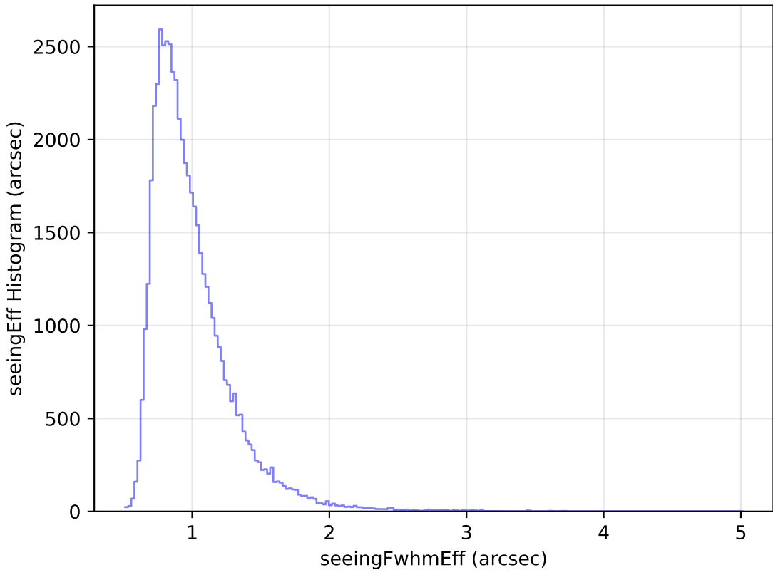
too_elab_r16_d2_giz_v3.4_10yrs Yr 1 i band: seeingEff Histogram
