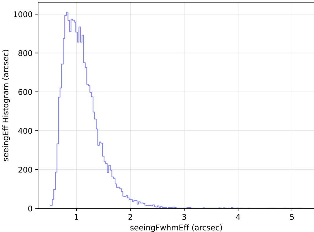
too_elab_r16_d2_giz_v3.4_10yrs Yr 1 g band: seeingEff Histogram
