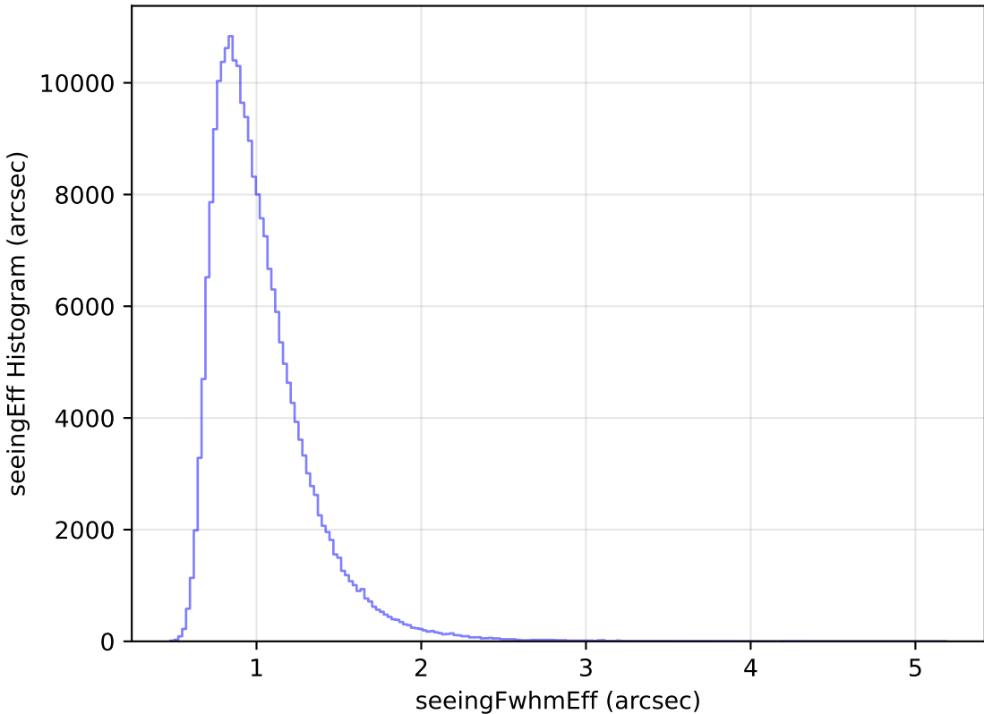
too_elab_r16_d2_giz_v3.4_10yrs Yr 1 all bands: seeingEff Histogram
