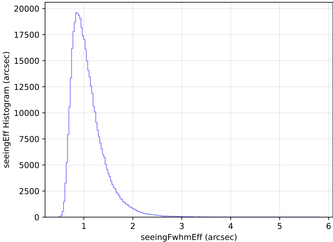
too_elab_r16_d2_giz_v3.4_10yrs WFD z band: seeingEff Histogram
