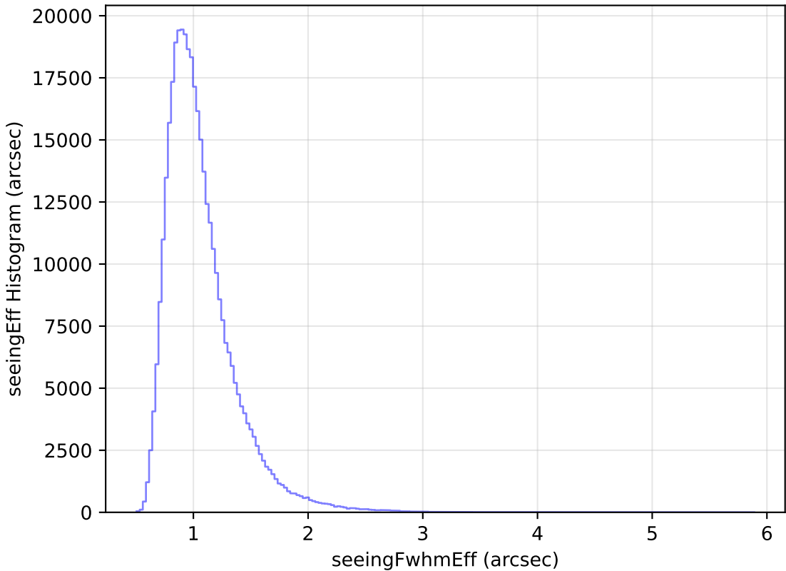
too_elab_r16_d2_giz_v3.4_10yrs WFD y band: seeingEff Histogram
