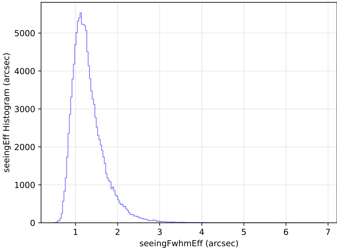
too_elab_r16_d2_giz_v3.4_10yrs WFD u band: seeingEff Histogram
