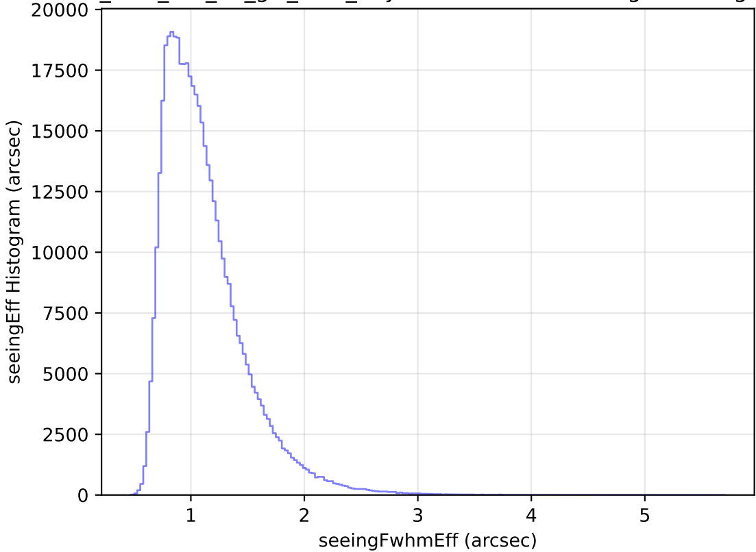
too_elab_r16_d2_giz_v3.4_10yrs WFD r band: seeingEff Histogram
