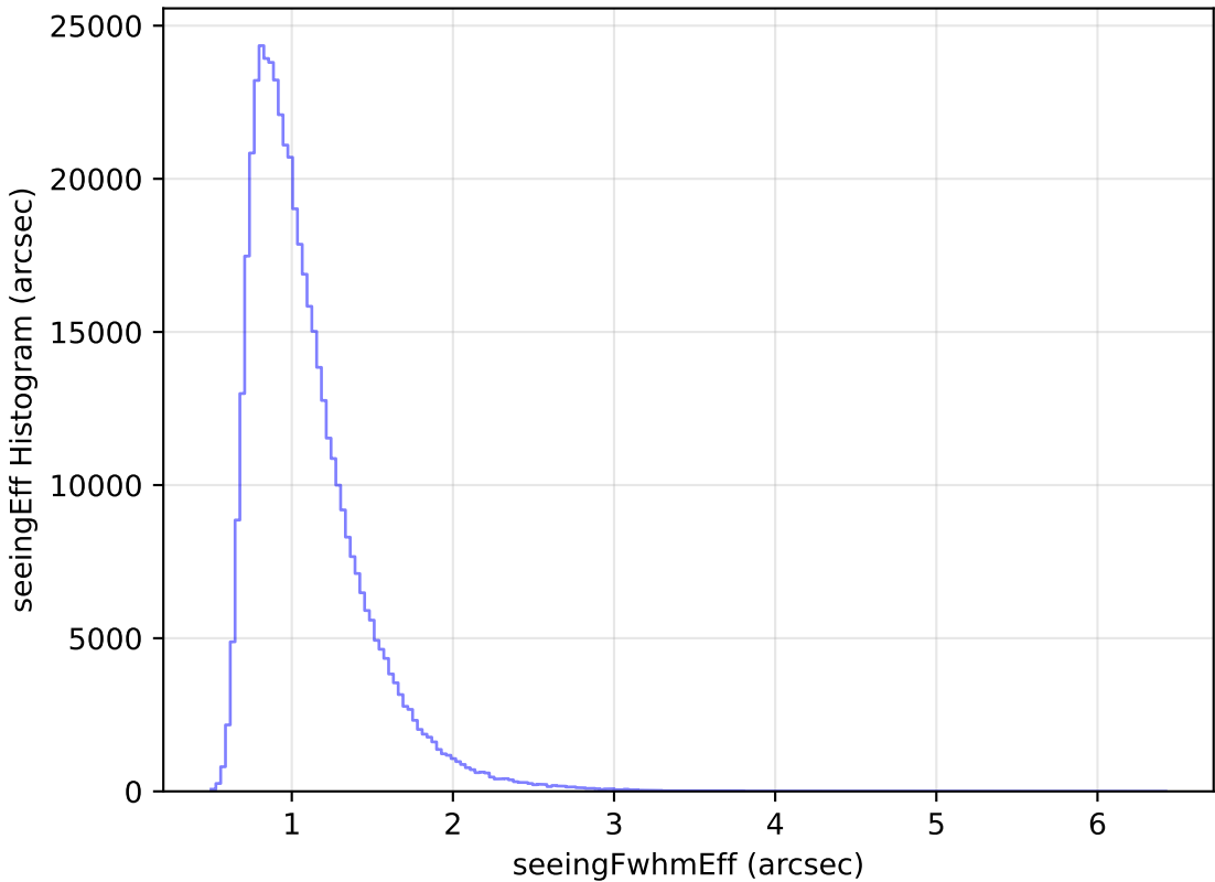
too_elab_r16_d2_giz_v3.4_10yrs WFD i band: seeingEff Histogram
