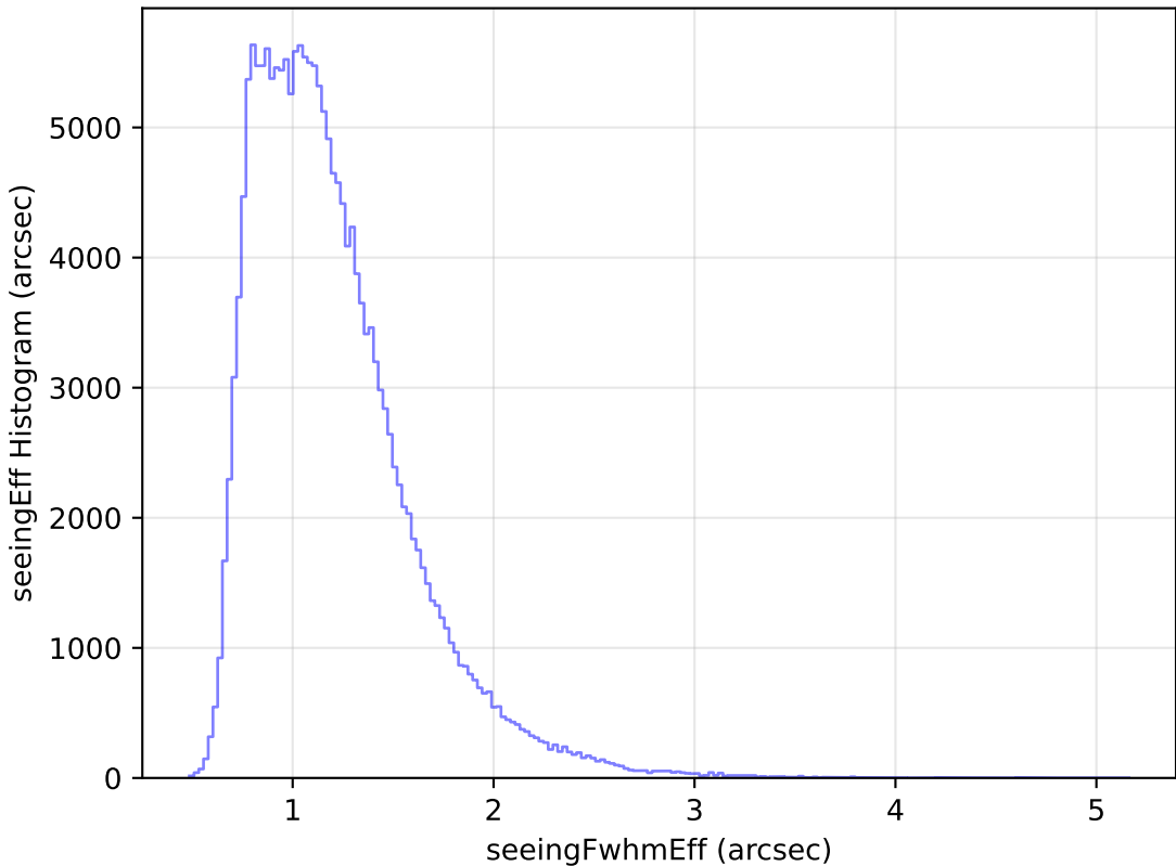
too_elab_r16_d2_giz_v3.4_10yrs WFD g band: seeingEff Histogram
