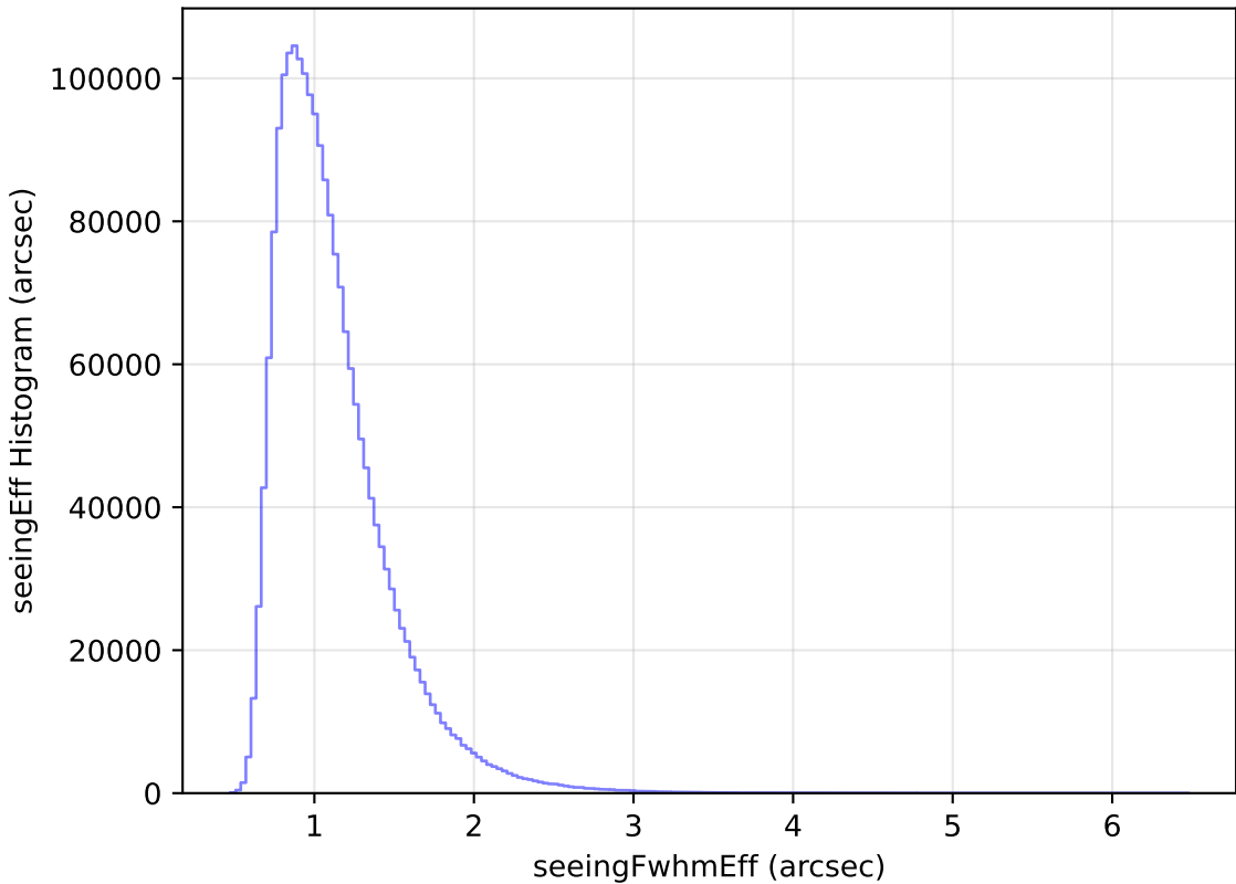
too_elab_r16_d2_giz_v3.4_10yrs WFD all bands: seeingEff Histogram
