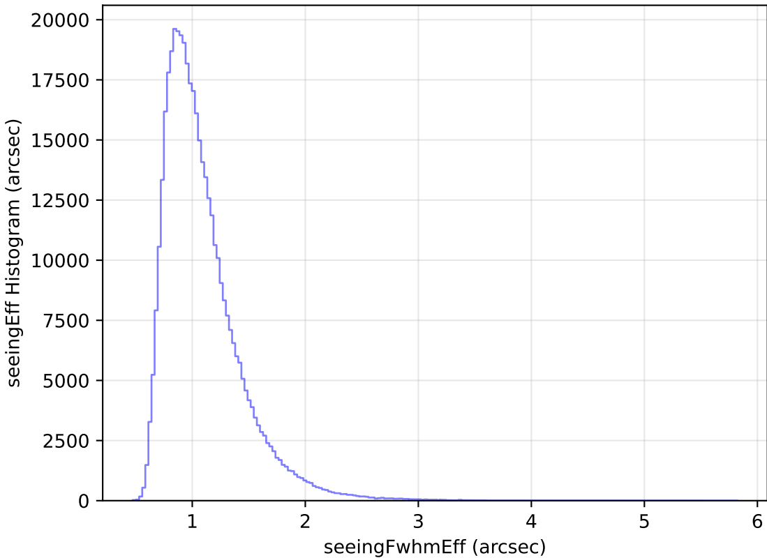
too_elab_r16_d2_giz_v3.4_10yrs All sky z band: seeingEff Histogram
