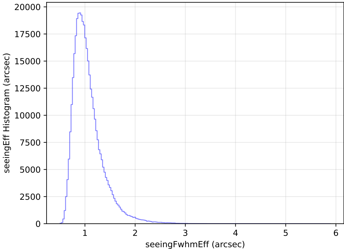
too_elab_r16_d2_giz_v3.4_10yrs All sky y band: seeingEff Histogram
