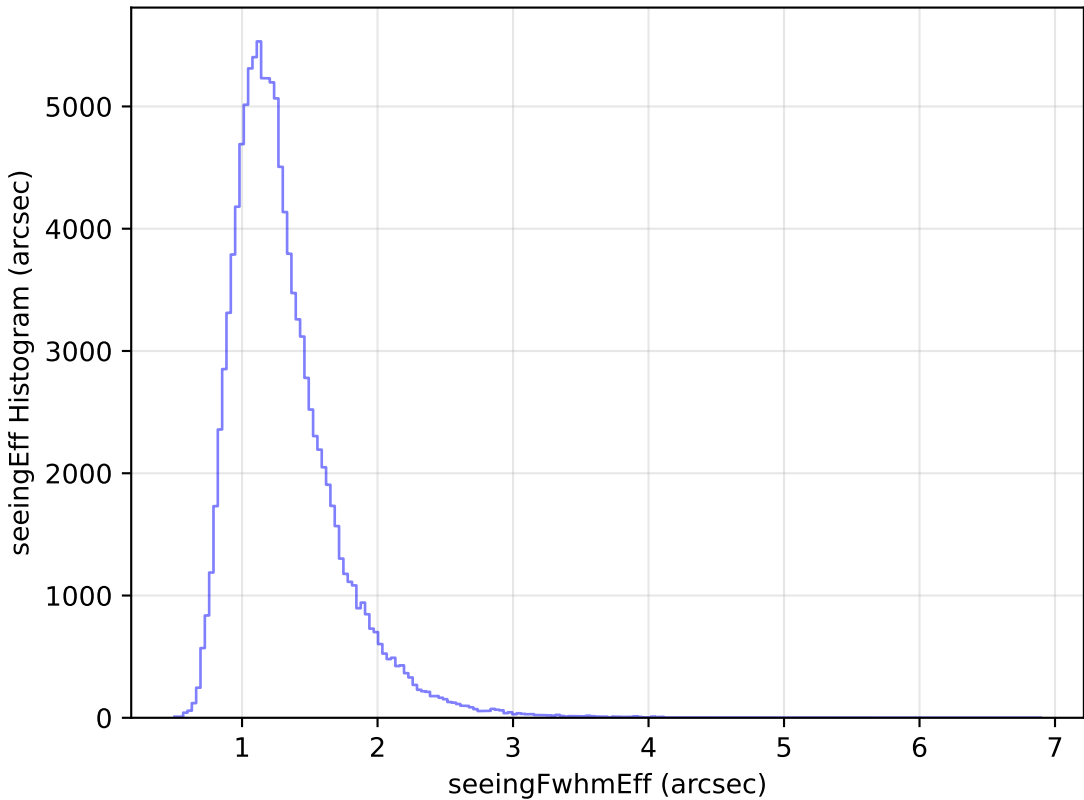
too_elab_r16_d2_giz_v3.4_10yrs All sky u band: seeingEff Histogram
