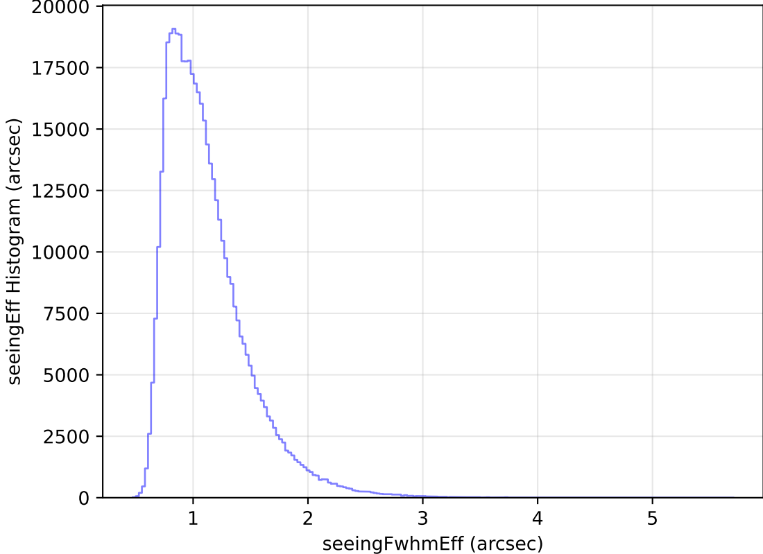
too_elab_r16_d2_giz_v3.4_10yrs All sky r band: seeingEff Histogram
