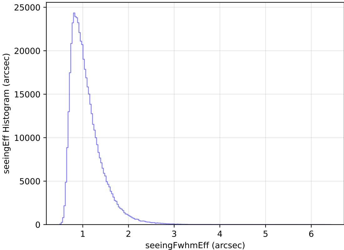
too_elab_r16_d2_giz_v3.4_10yrs All sky i band: seeingEff Histogram
