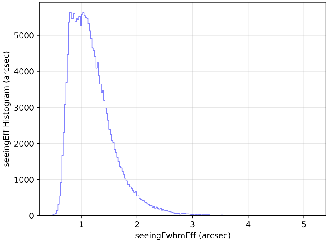
too_elab_r16_d2_giz_v3.4_10yrs All sky g band: seeingEff Histogram
