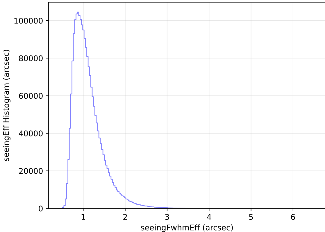
too_elab_r16_d2_giz_v3.4_10yrs All sky all bands: seeingEff Histogram
