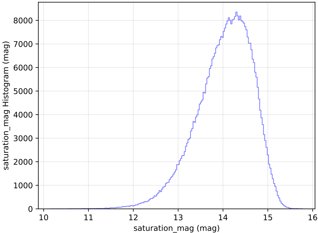
too_elab_r16_d2_giz_v3.4_10yrs WFD z band: saturation_mag Histogram
