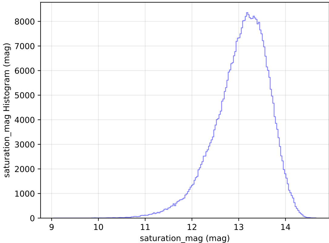
too_elab_r16_d2_giz_v3.4_10yrs WFD y band: saturation_mag Histogram
